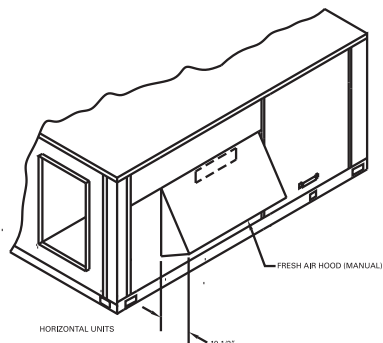
Figure 7. Fresh air hood (horizontal units)
