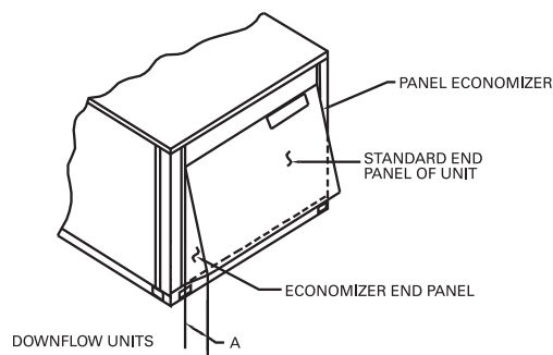
Figure 12. Economizer - downflow units
