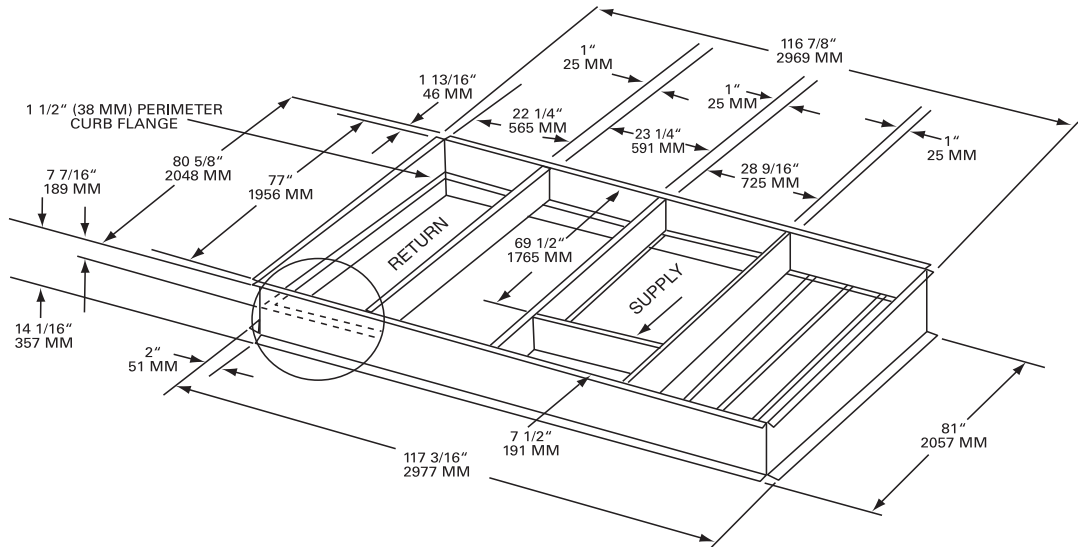
Figure 3. Heat pump models - 12½ - 20 tons
