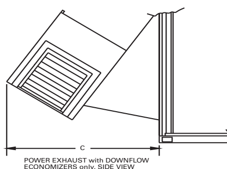
Figure 10. Power exhaust - downflow economizers - side view
