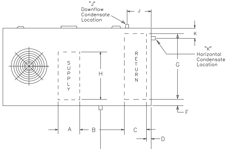
Figure 6. Downflow & horizontal condensate locations
