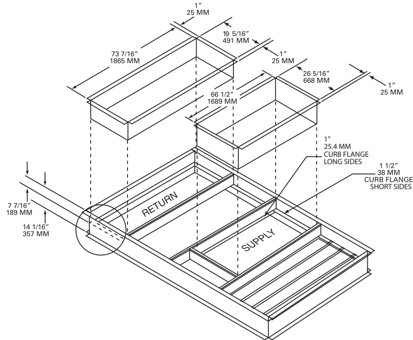
Figure 4. Heat pump models - 12½ - 20 tons
