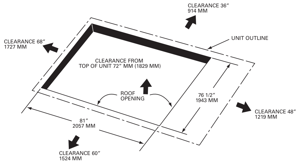
Figure 5. Heat pump models - 12½ - 20 tons
