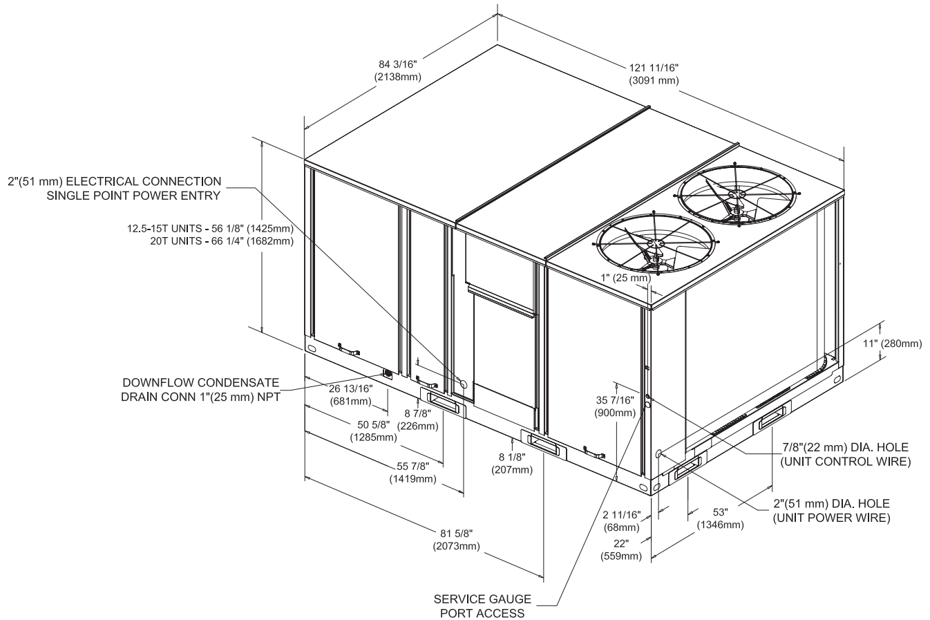
Figure 1. Heat pump models - 12½ - 20 tons
