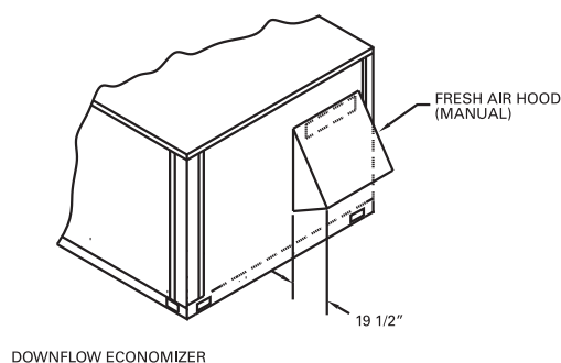
Figure 8. Fresh air hood (downflow units)
