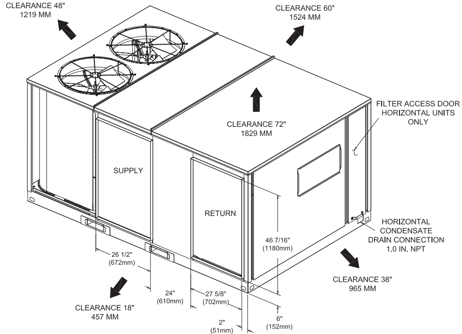
Figure 2. Heat pump models - 12½ - 20 tons
